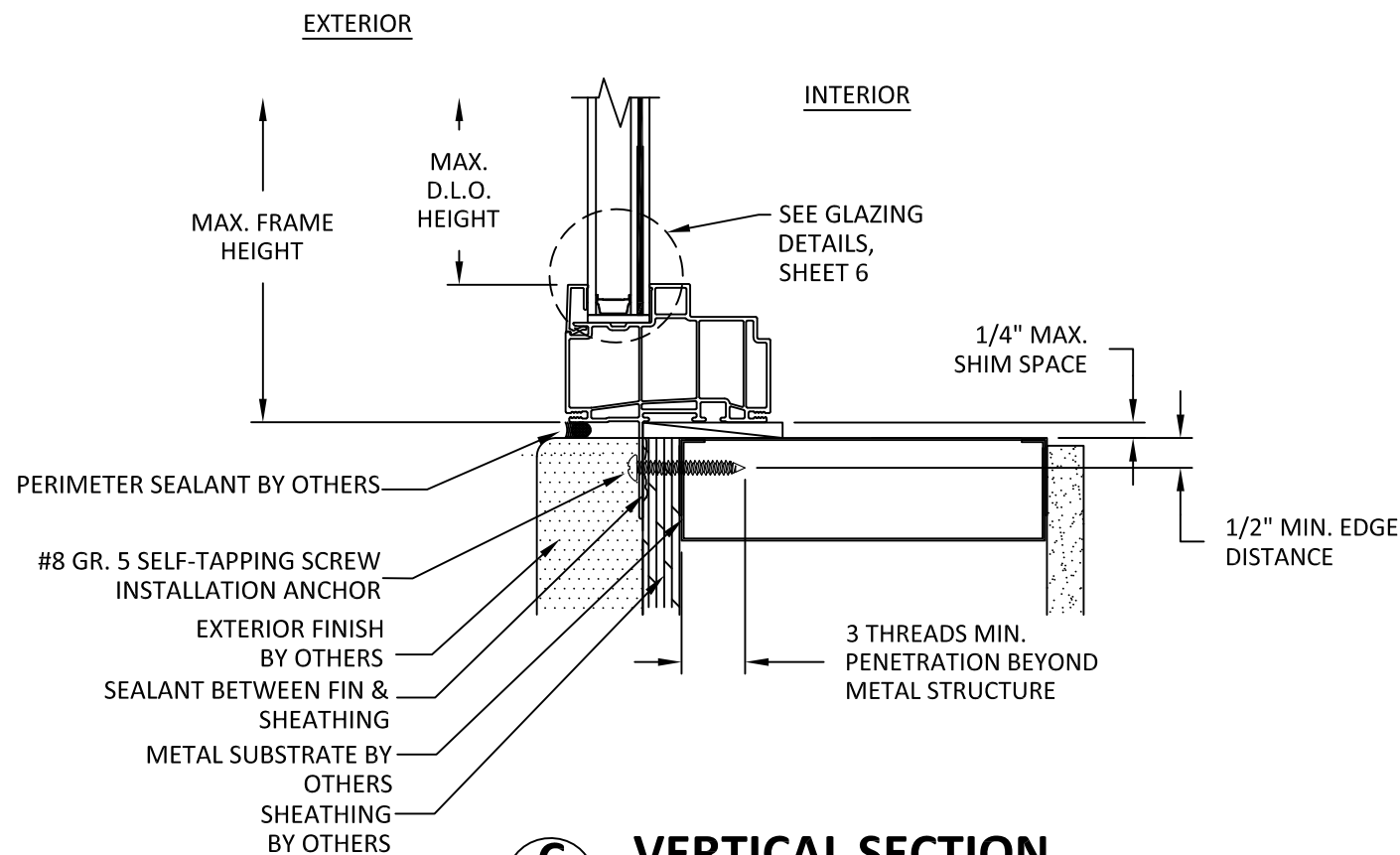
C 4 VERTICAL SECTION NAIL FIN INSTALLATION METAL SUBSTRATE
