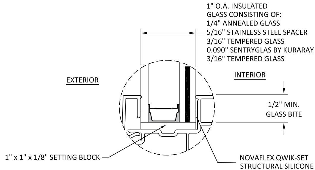
GLAZING DETAIL 1
