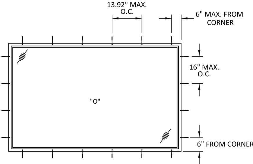
TYPICAL ANCHOR LAYOUT CLIP INSTALLATION
