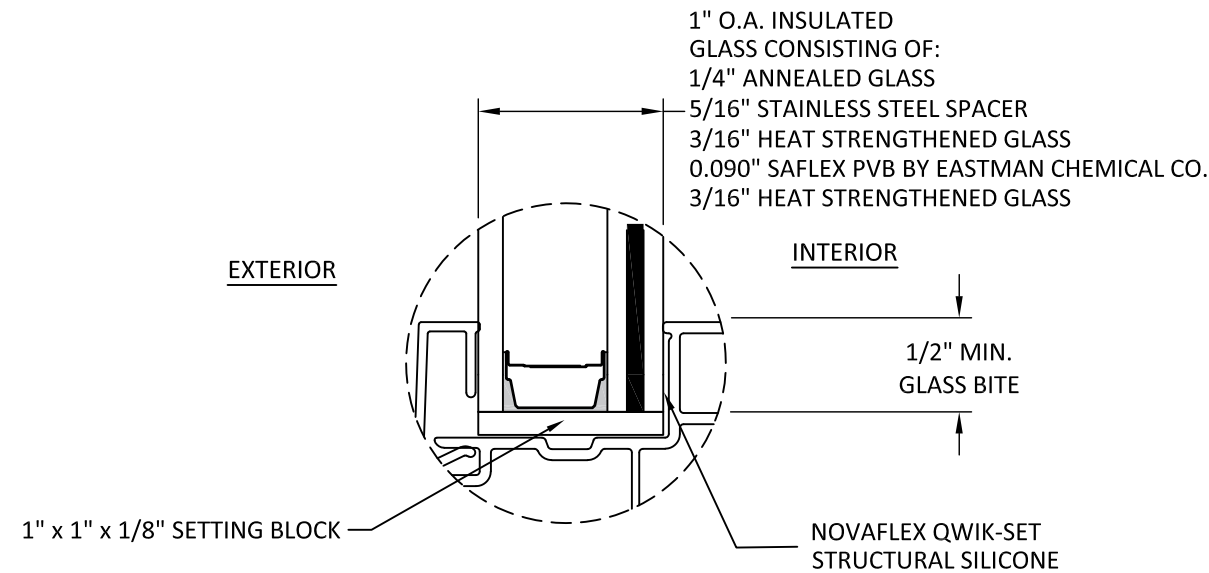
GLAZING DETAIL 2
